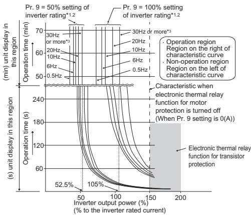
Electronic thermal relay function operation characteristic
